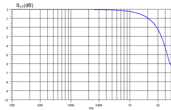
Figure 7. S 21 attenuation
